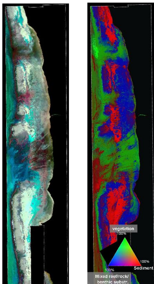
Figure 7 HyMap derived bottom reflectance corrected for depth and water body properties (left). General classification of the three main seafloor coverage groups (right).
