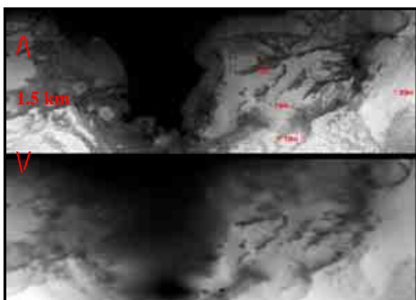
Figure 5 HyMap derived bathymetry subset (top) and comparison to gridded echo sounding derived map.
