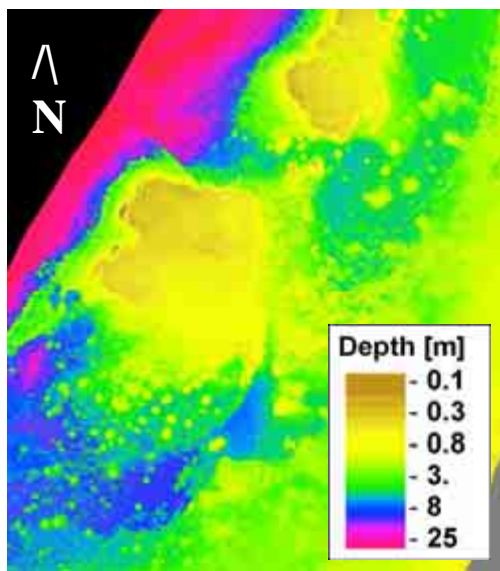
Figure 9 Subset of Fig. 8b, demonstrating the spatial resolution of 3.2m pixel size and show the seamless mapping.
