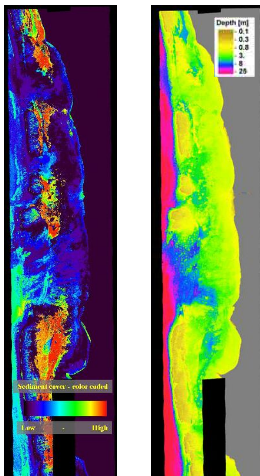
Figure 8 HyMap derived sediment cover (colour coded) on the left (a) and HyMap derived bathymetry with colour chart on the right (b).
