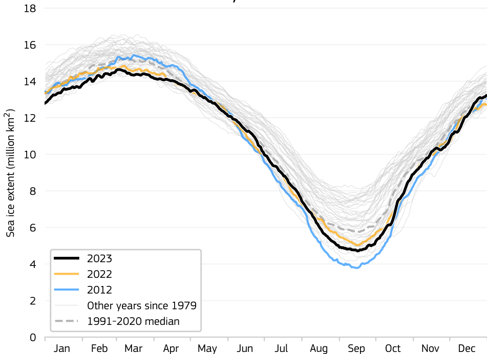
Daily sea ice extent
