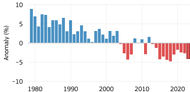
Anomalies in sea ice extent for March
