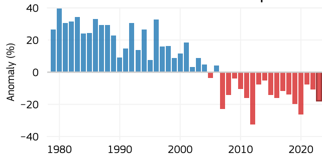
Anomalies in sea ice extent for September
