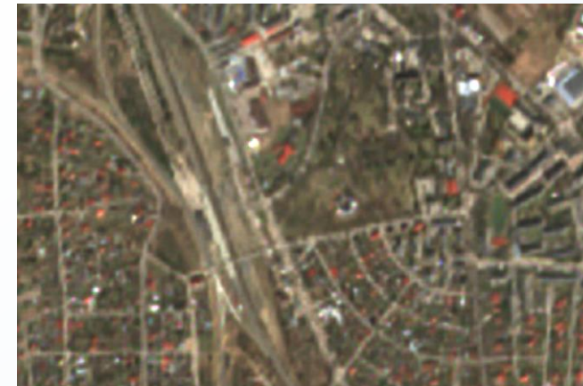
Sentinel-2 imagery +s2enh 2.5 m resolution
