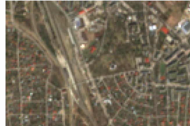
Sentinel-2 imagery 10 m resolution
